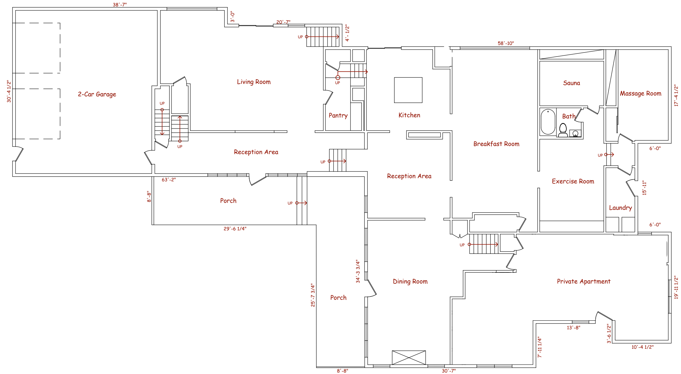
1. LEVEL 1 PLAN SCALE 1" : 10" 1" = 10" 0 10' 20'
